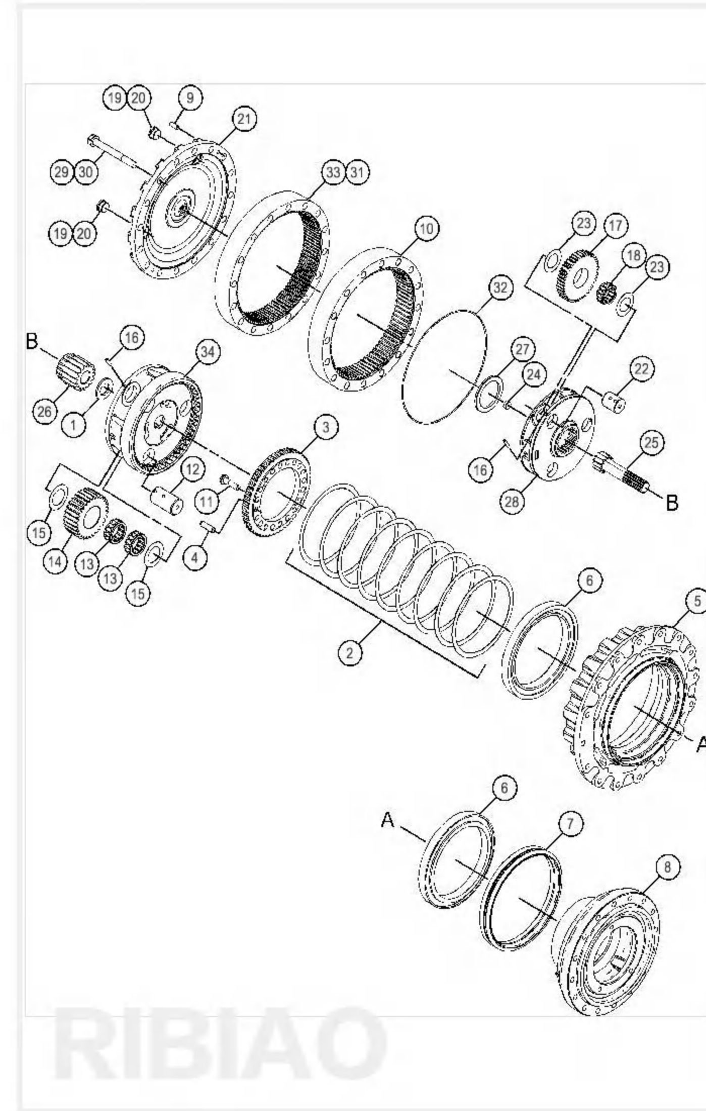
行走齿圈 Ring gear, Travel
