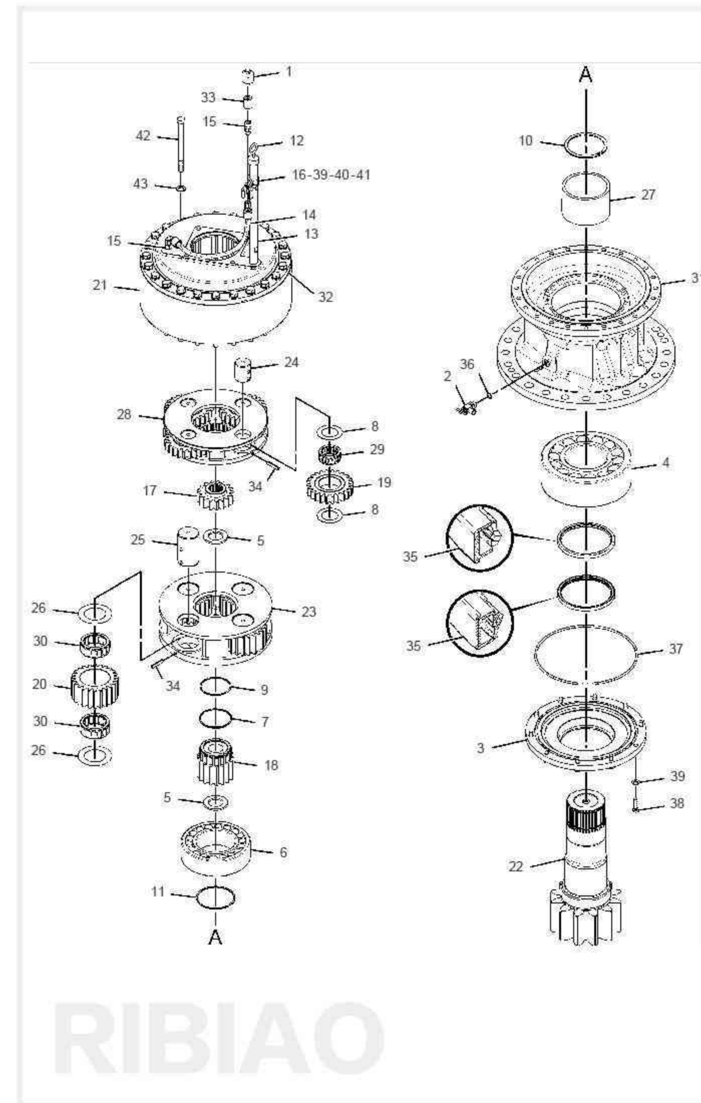
回转齿圈 Ring gear,Swing
